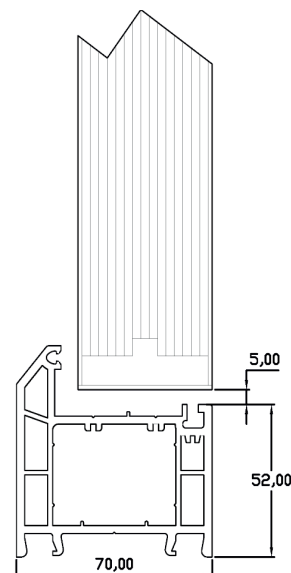
72mm PVC
