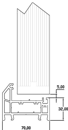
52mm PVC
